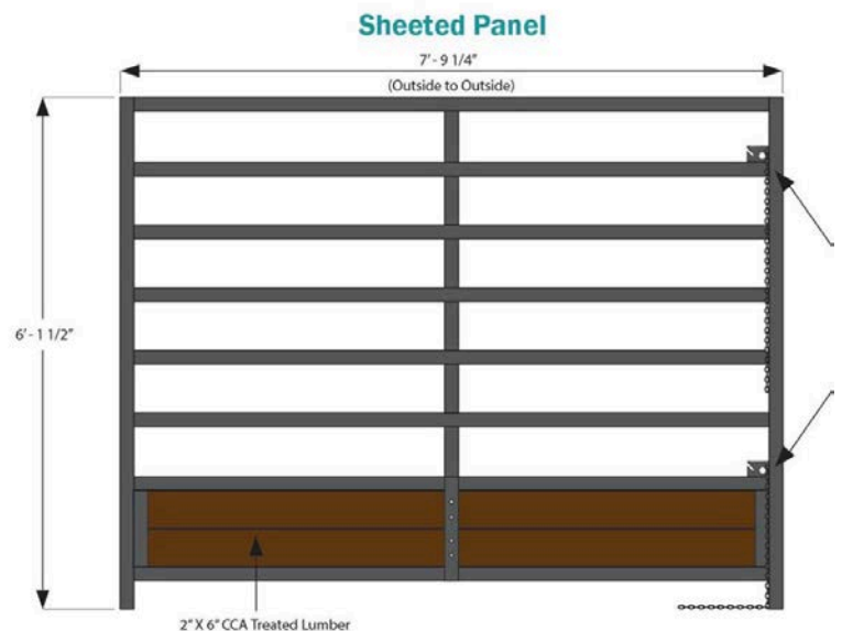
Panel Dimensions
